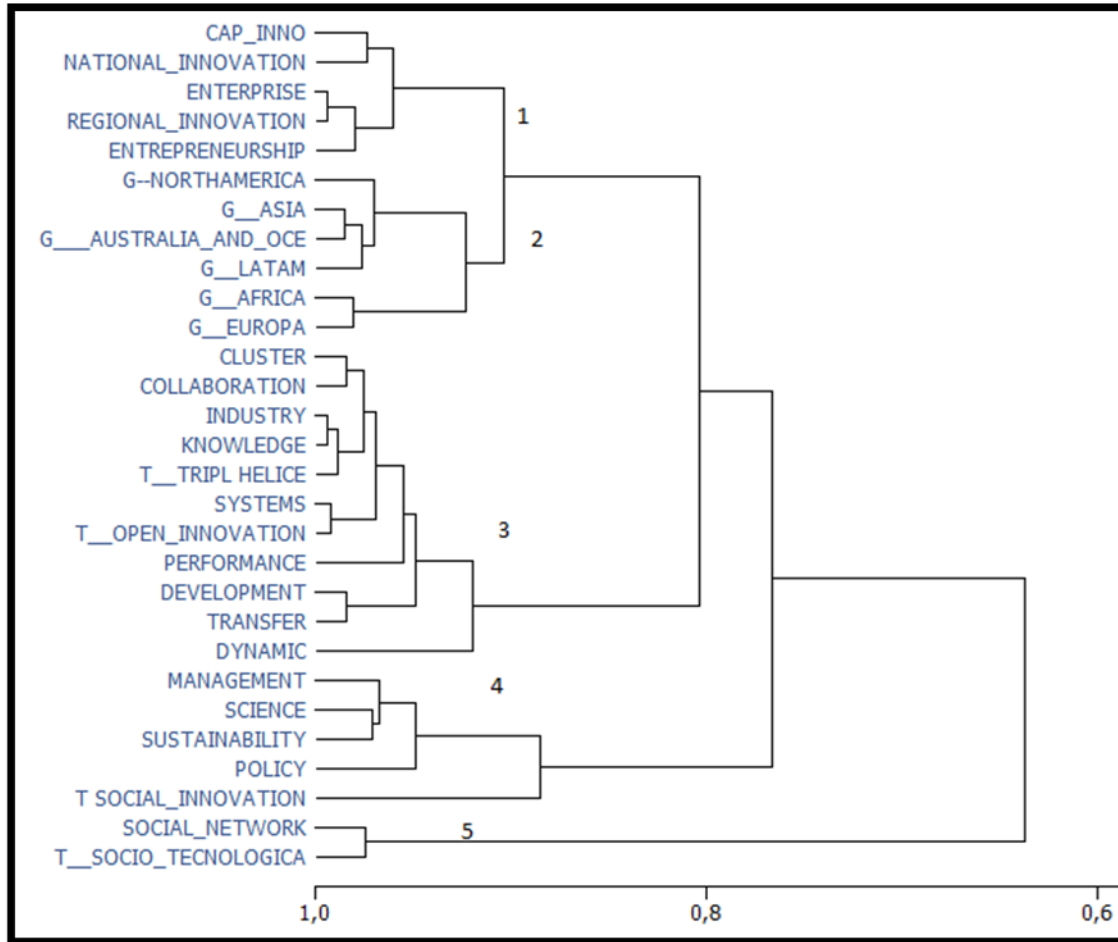
Figure 1: Dendrogram based on Similarity Index. Source: Own elaboration. (Wordstat/ Heatmap / Keyword dendogram).
